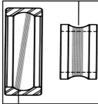
Typical wear pattern of bearing with misalignment. Bearing will have wider path or wear path running from one side of race to the other.
