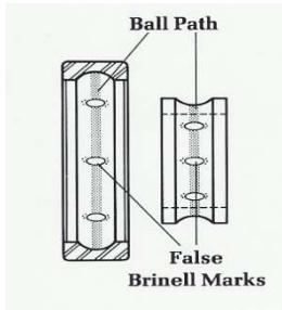
Typical appearance of a bearing subject to fretting wear
