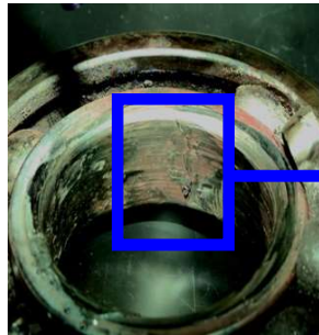
Fretting can occur on the inner ring of bearings where they meet the shaft
