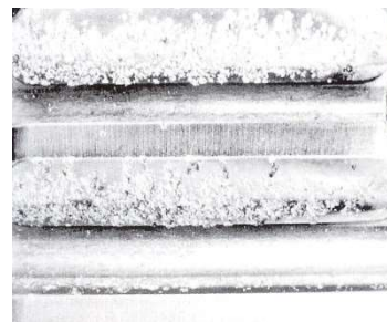
Current sparkover craters in the raceway of a bearing and on a gear surface
